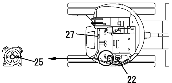
グリル内側詳細 DETAILS OF GRILLE INSIDE
